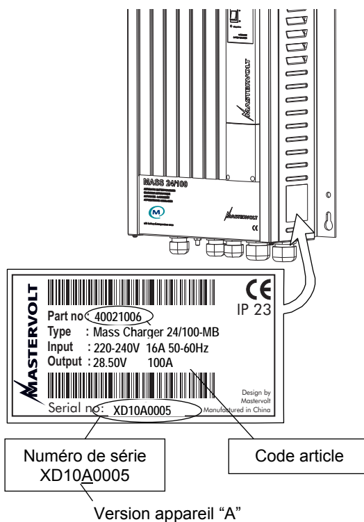
Figure 1: Plaque d'identification
